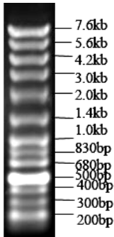
0.8% agarose gel
